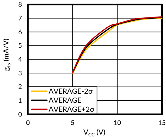
Figure 3. Typical forward transconductance as a function of supply voltage at T amb =25°C
