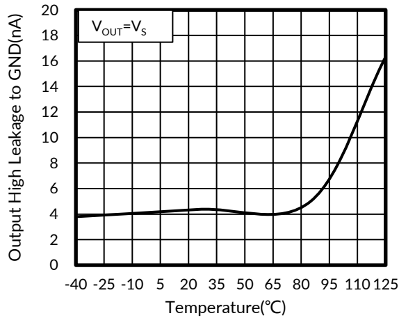
Figure 19. Output High Leakage Current vs Temperature at 5V
