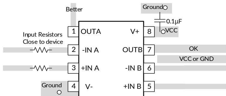
Figure 31. LM2903H Layout Example
