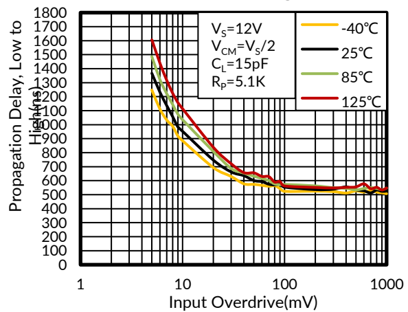
Figure 24. Low to High Propagation Delay vs Input Overdrive Voltage, 12V
