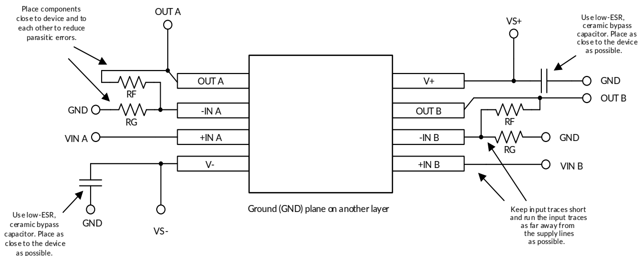
Figure 29. Layout Example
